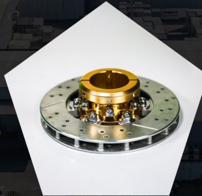
Floating Brake Rotor
